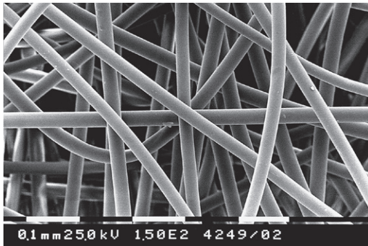
Figure 1 Magnified mechanically bonded nonwoven [1]
