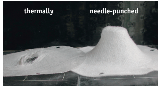
Figure 5 Typical behaviour of 200g/m² needle-punched and thermally bonded nonwovens in the plunger puncture test (simulation of a stone puncture)
