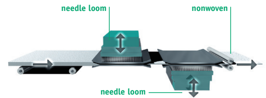
Figure 2 Needle-punched nonwoven process
