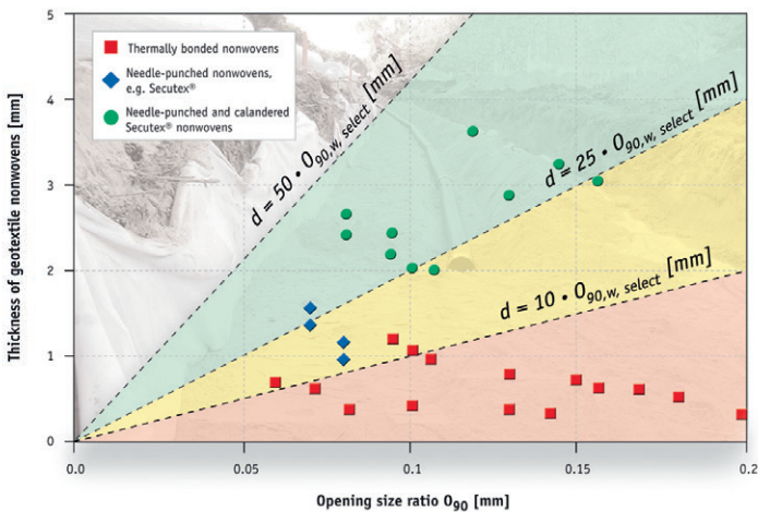
Figure 8 Recommended opening size and thickness correlation for a filter geotextile (DVK, Vol. 221/1992)
