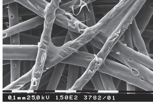
Figure 4 Thermally bonded nonwoven [1]
