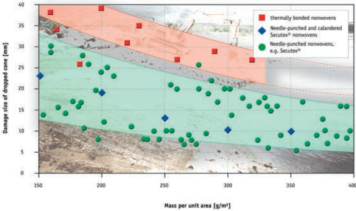
Figure 7 Cone drop behaviour (according to EN ISO 134333) of thermally bonded and needle-punched nonwovens
