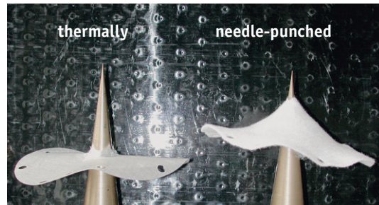
Figure 6 Typical behaviour of 200g/m² needle-punched and thermally bonded nonwovens in the cone drop test (simulation of a puncture load)
